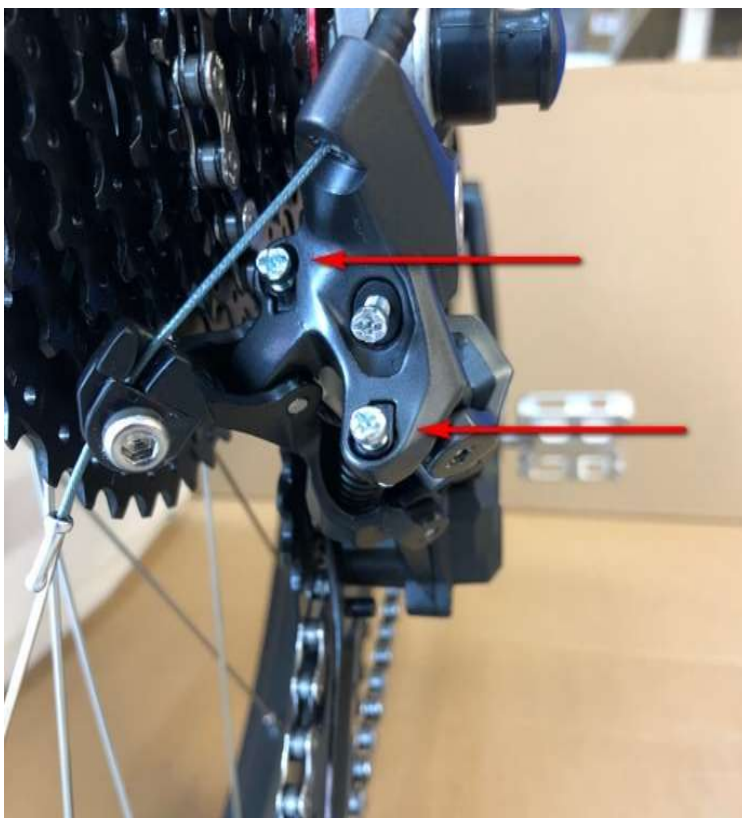
Upper arrow: (H) End stop of 10th gear Lower arrow: (L) End stop of the 1st gear
