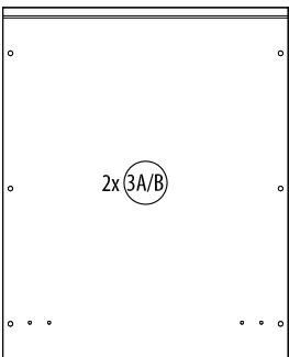
2-6669 472x580x19mm
