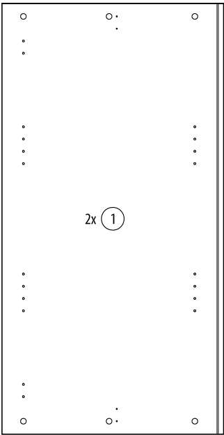
2-6663 1124x579x19mm
